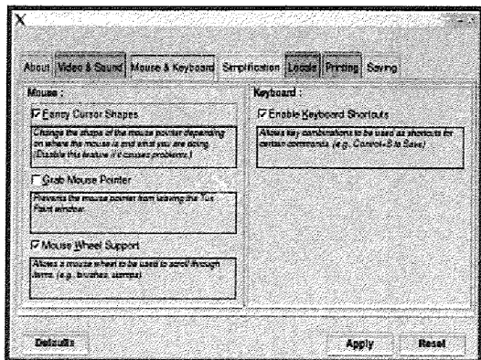
Tux Paint Config, graphical configuration tool for parents and teachers.
